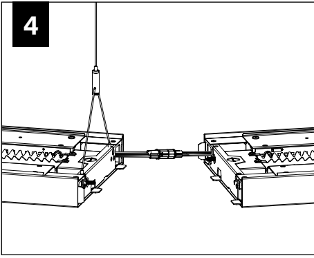
4 MAKE ELECTRICAL CONNECTION
