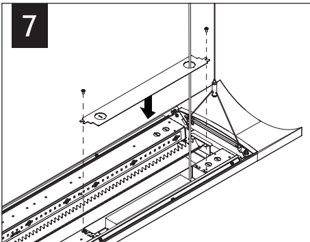
JOINED RUNS
