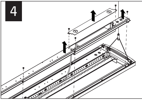
JOINED RUNS
