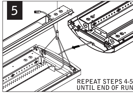
JOINED RUNS
